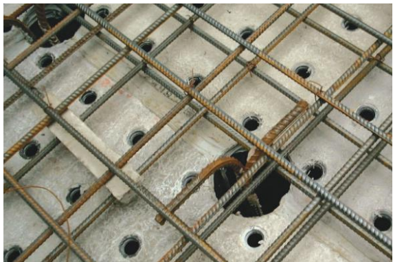
Steel reinforcement showing connecting steel within column form
